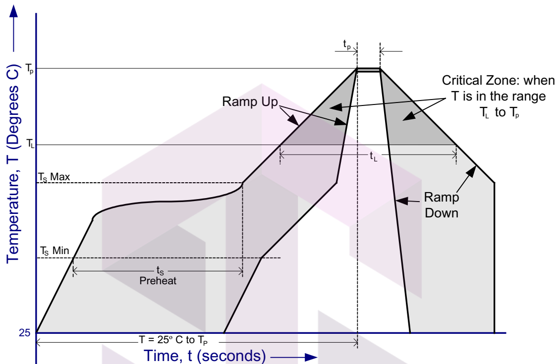
Figure 10 - FT232R Solder Reflow Profile
